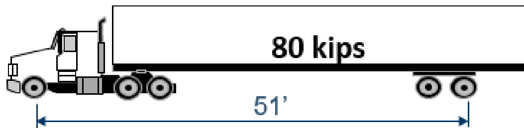
Type M3S2-40
